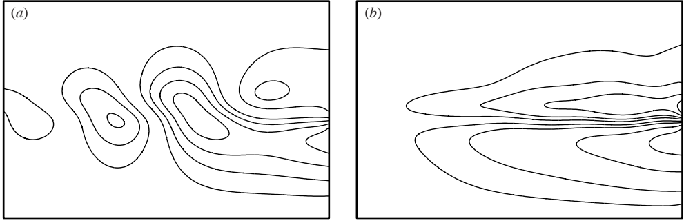
FIGURE 13. Simulation of a transient shear layer. (a) Instantaneous fluctuation streamlines at time t/T = 11/8 , where T is the period. (b) Shift mode which is added to the Galerkin approximation (2.14) as fifth mode and describes the difference between the initial parallel flow and the averaged post-transient flow, modulo the orthonormal correction with respect to the first Karhunen–Loève modes.
